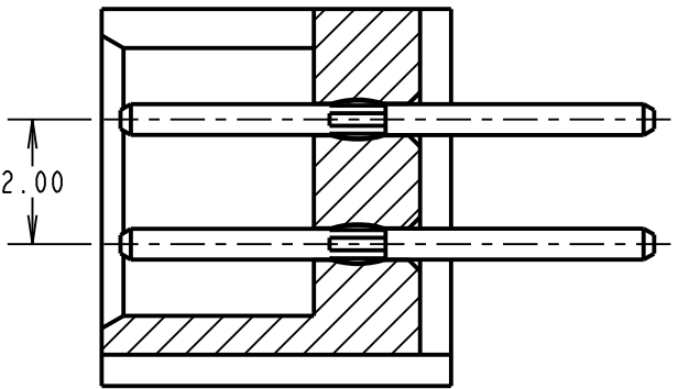
SECTION X-X
